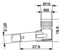
Dimensioned drawing
