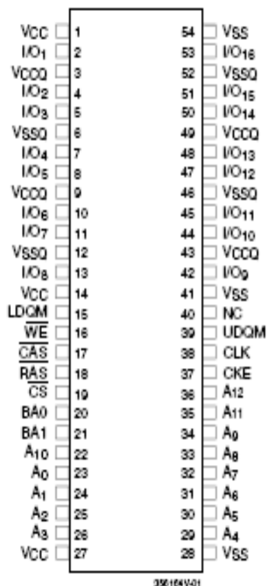
54 Pin Plastic TSOP-II x16 PIN CONFIGURATION Top View
