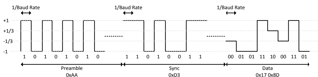
Figure 18: Data Sent Over the Air (MDMCFG2.MOD_FORMAT=100)
