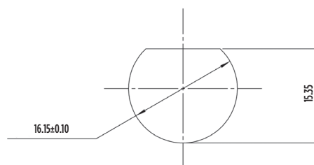
PANEL CUT-OUT DETAIL
