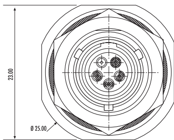
FRONT FACE
