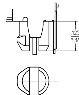
PEG DETAIL SCALE 8:1
