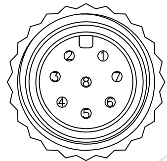
Conn.1 Pin Assignments Front View
