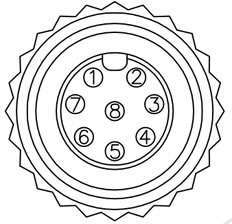
Conn.2 Pin Assignments Front View
