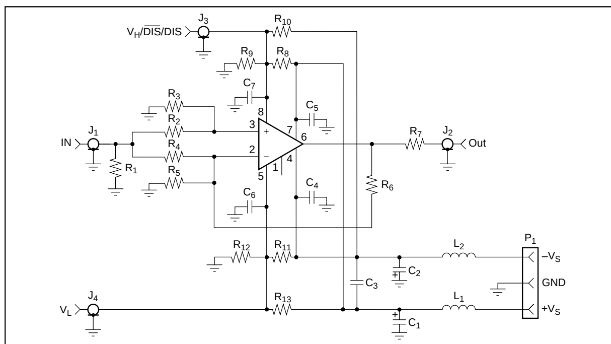
FIGURE 2. Circuit Schematic for DEM-OPA68xU.
