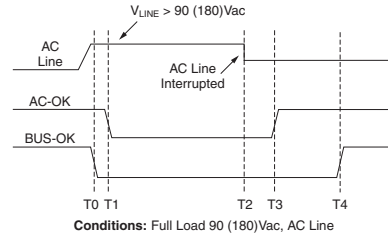
Conditions: Full Load 90 (180)Vac, AC Line
