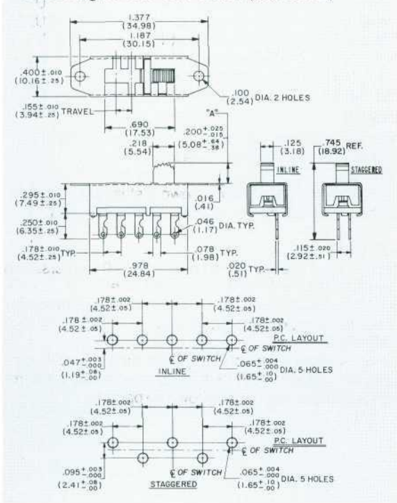
G-140 Single Pole/Four Position (with detent)
