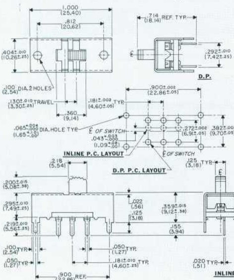
GPF-124 Single Pole Double Throw (with detent) GPF-126 Double Pole Double Throw (with detent)
