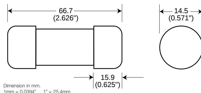
Fig. 1: 20-30 Amp Range
