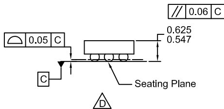
SIDE VIEWS
