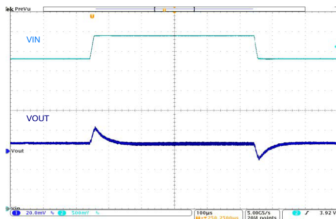
Figure 13. Line Transient, 3.6\text{--}4.2\text{ V}_{IN} , 1.15625\text{ V}_{OUT} , 10\text{ }\mu\text{s} Edge at 1 A Load
