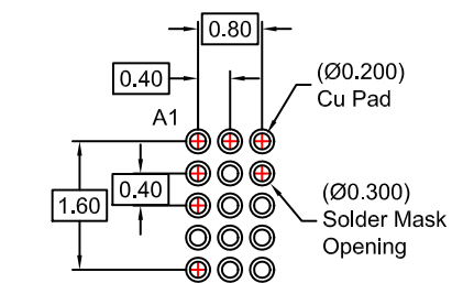
RECOMMENDED LAND PATTERN (NSMD TYPE)
