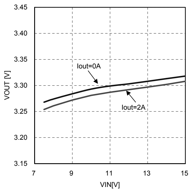
Figure 9. VOUT Line Regulation ( V_{\text{OUT}}=3.3\text{V} , L=3.3\mu\text{H} , I_{\text{out}}=0\text{A} / 2\text{A} )
