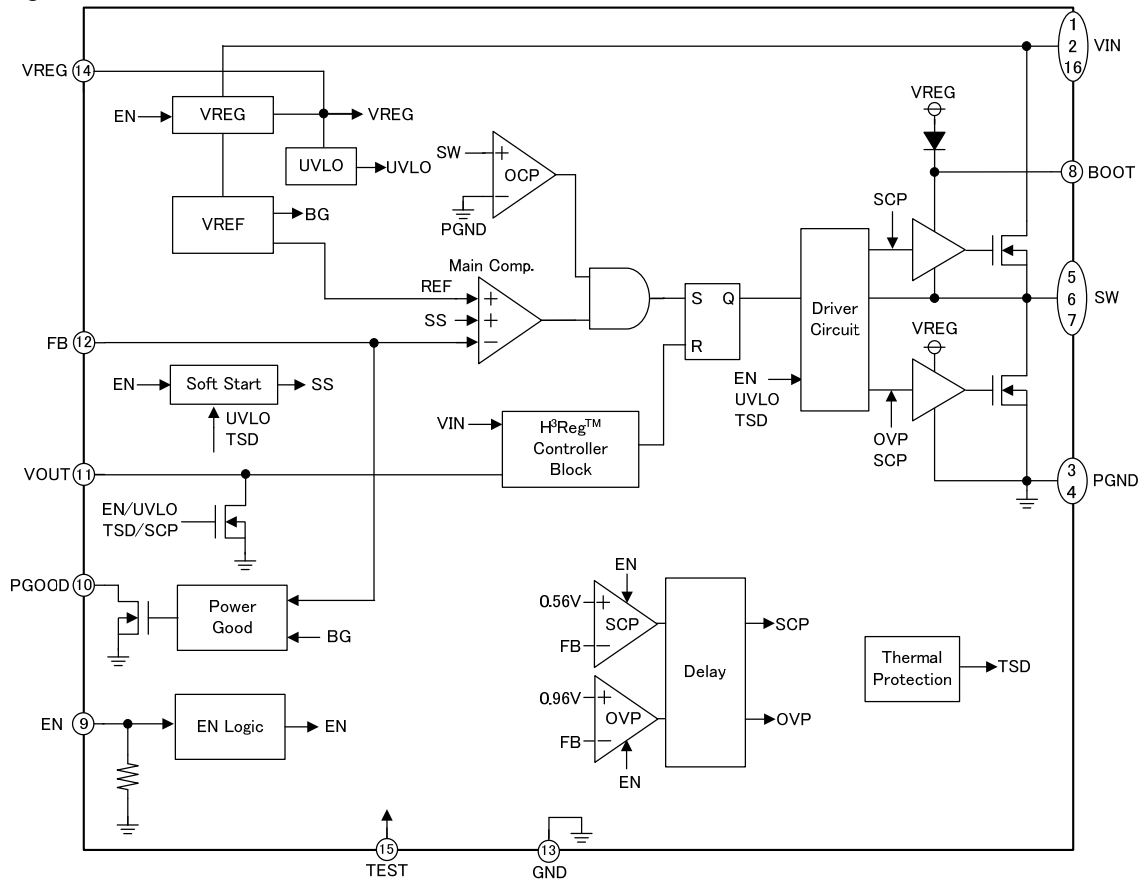
Figure 3. Block Diagram
