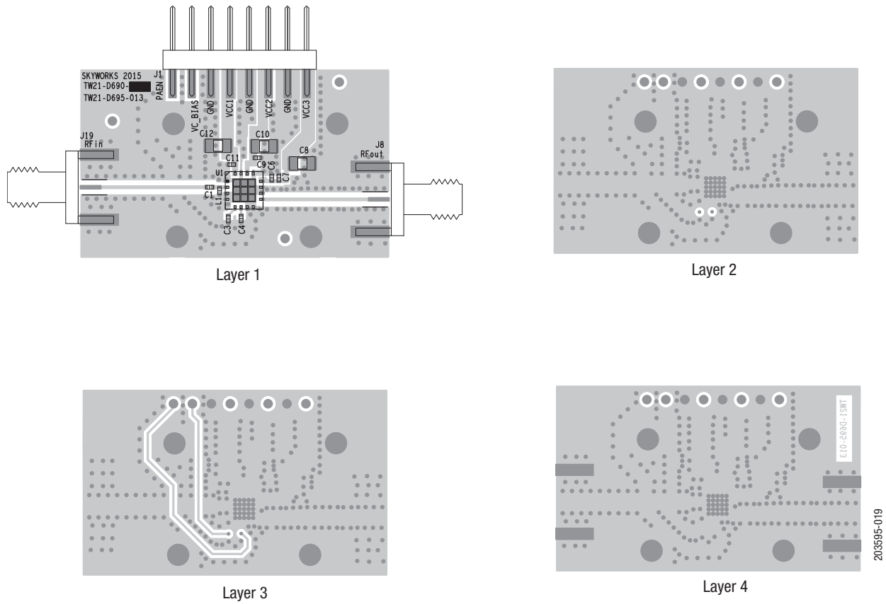
Figure 19. Evaluation Board Layer Details
