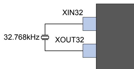
Figure 44-6. External Real Time Oscillator without Load Capacitor
