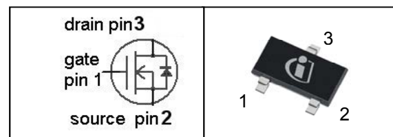
PG-SC-59
