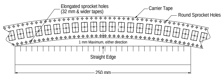
Figure 8 – Maximum Camber
