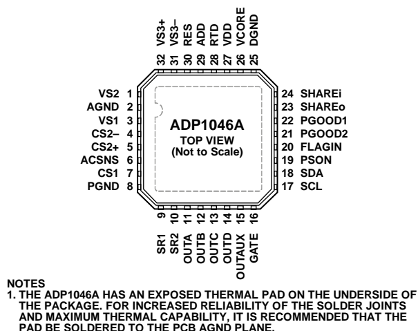
Figure 3. Pin Configuration
