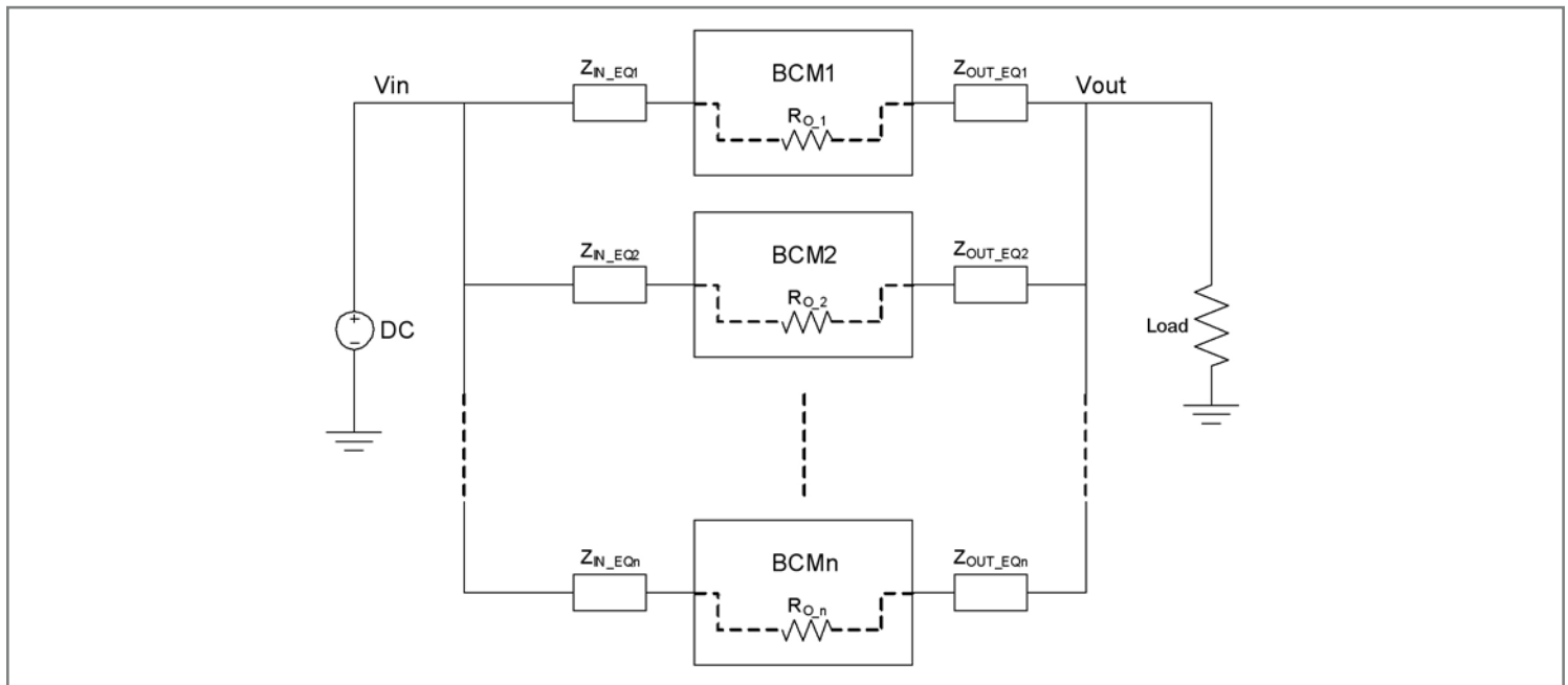
Figure 18 – BCM Array
