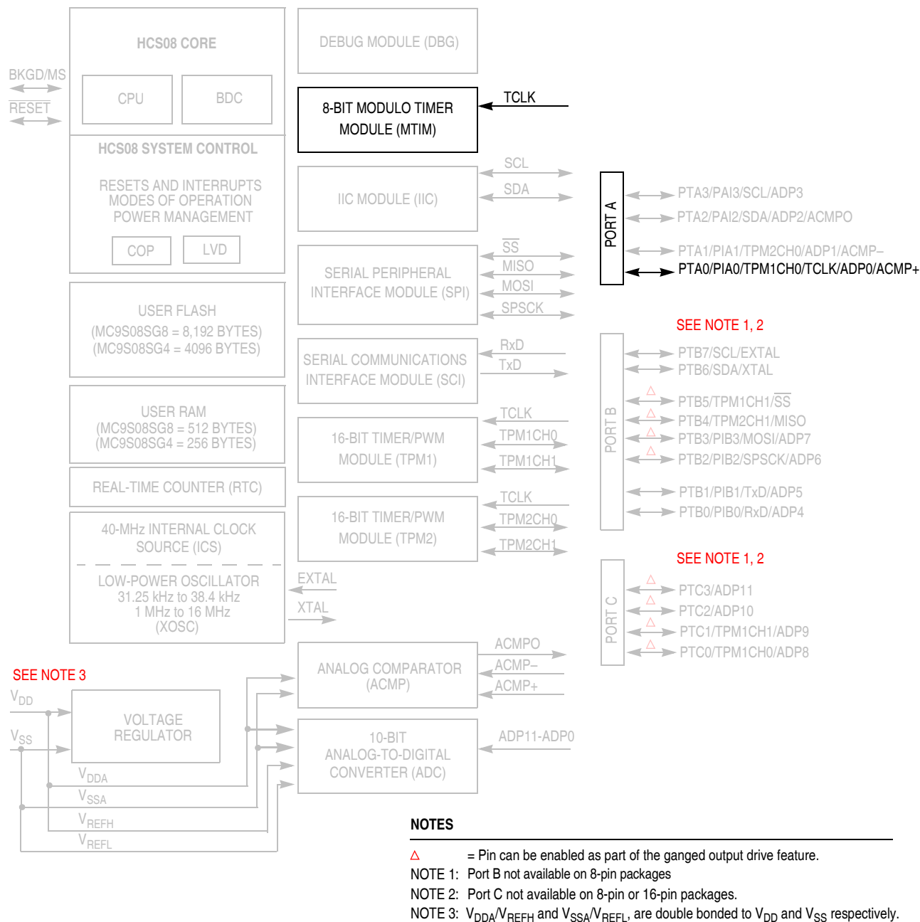
Figure 12-1. MC9S08SG8 Block Diagram with MTIM Module Highlighted
