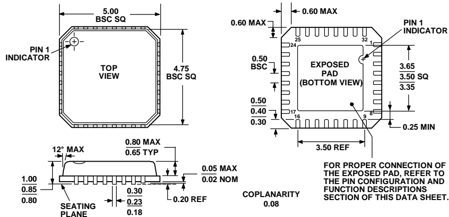
COMPLIANT TO JEDEC STANDARDS MO-220-VHHD-2 Figure 55. 32-Lead Lead Frame Chip Scale Package [LFCSP_VQ] 5 mm × 5 mm Body, Very Thin Quad (CP-32-4) Dimensions shown in millimeters
