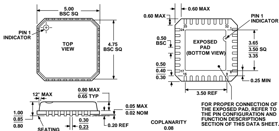
Figure 55. 32-Lead Lead Frame Chip Scale Package [LFCSP_VQ] 5 mm x 5 mm Body, Very Thin Quad (CP-32-4) Dimensions shown in millimeters
