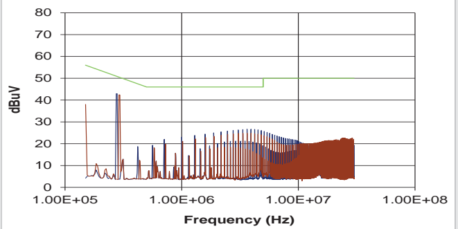
NXJ2S1212MC (Average)
