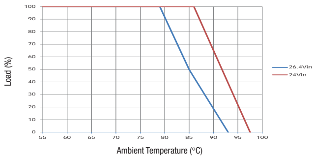
NXJ2S2415MC
