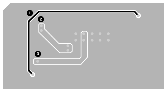
Figure 16. Top Layer of an Example Layout for an ADP1864 Application
