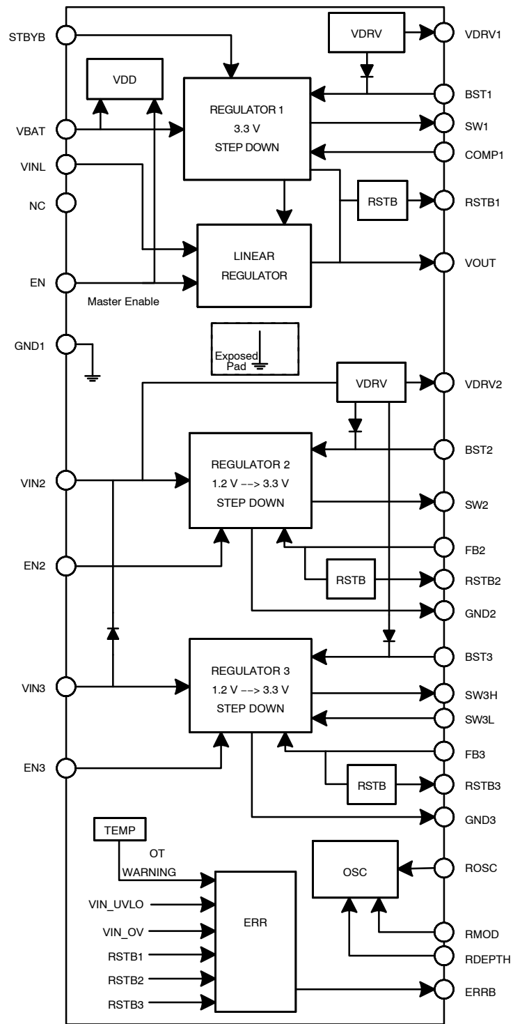
Figure 2. NCV97311 Block Diagram – 3.3 V Version
