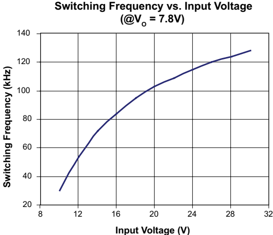
Fig. 9. Switching Frequency vs. Input Voltage Plot
