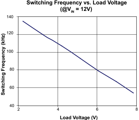
Fig. 9. Switching Frequency vs. Load Voltage Plot
