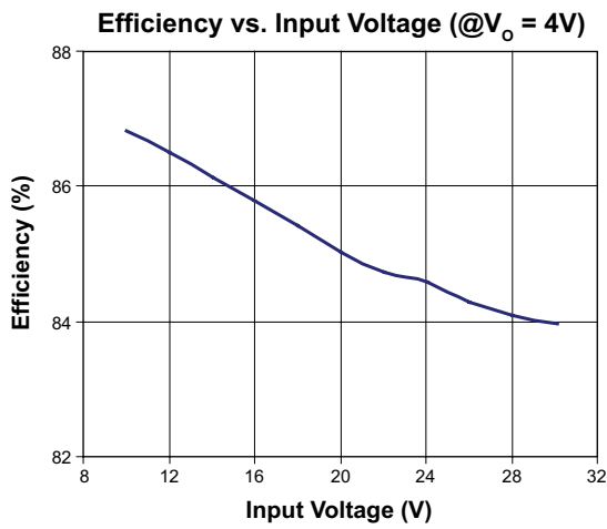
Fig. 1. Efficiency vs. Input Voltage Plot
