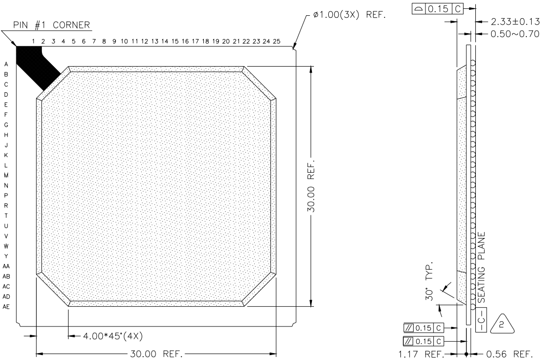
Figure 26: 313 PBGA - Top and Side View
