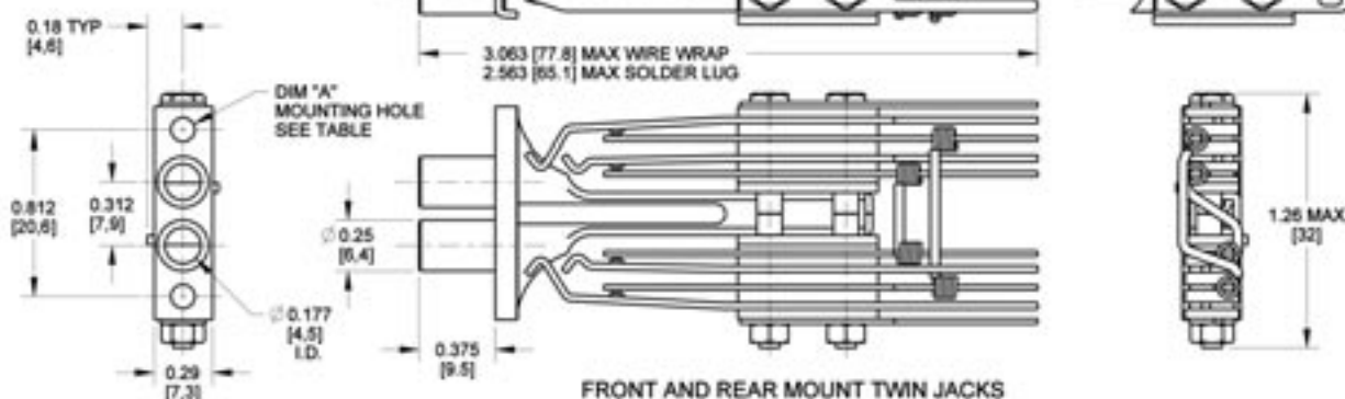
FRONT AND REAR MOUNT TWIN JACKS
