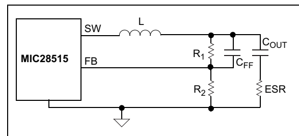
FIGURE 5-3: Inadequate Ripple at FB.
