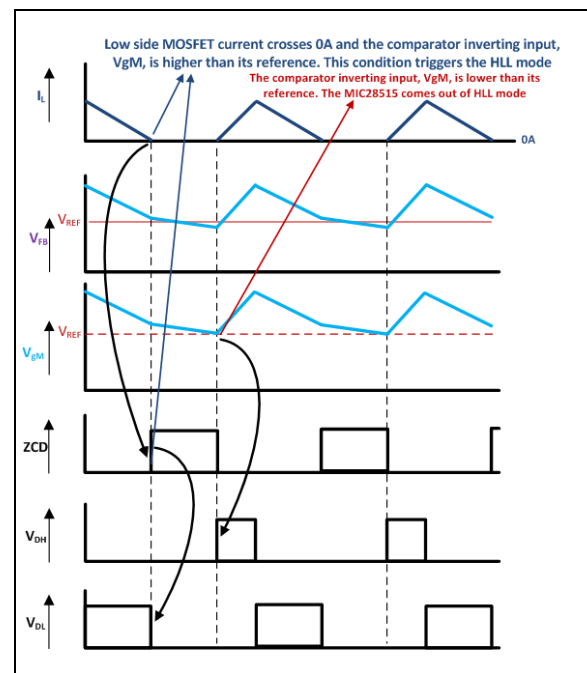
FIGURE 4-3: MIC28515 Control Loop Timing (HLL Mode).
