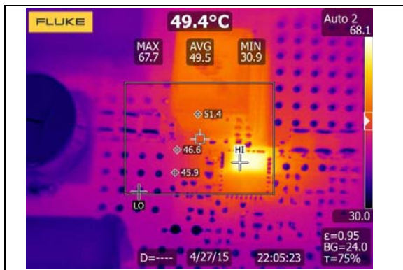
FIGURE 2-51: Thermal Picture ( I_{OUT} = 5A ).
