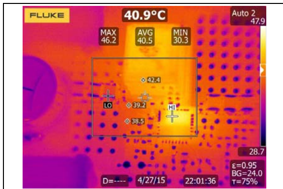
FIGURE 2-50: Thermal Picture ( I_{OUT} = 2.5A ).
