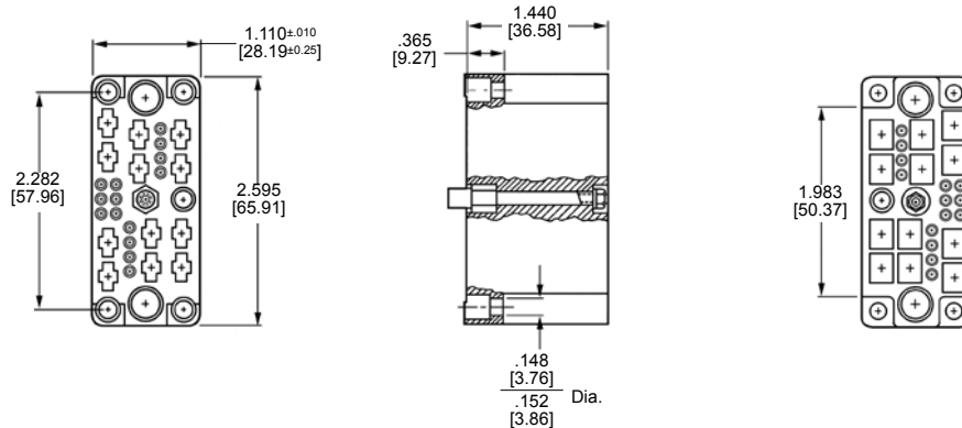
Receptacle Housing
