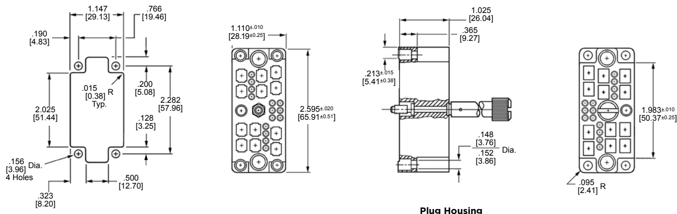
Plug Housing
