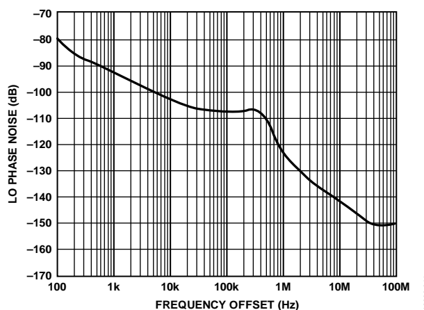
Figure 140. LO Phase Noise vs. Frequency Offset, LO = 3800 MHz, PLL Loop Bandwidth = 300 kHz, Spectrum Analyzer Limits Far Out Noise
