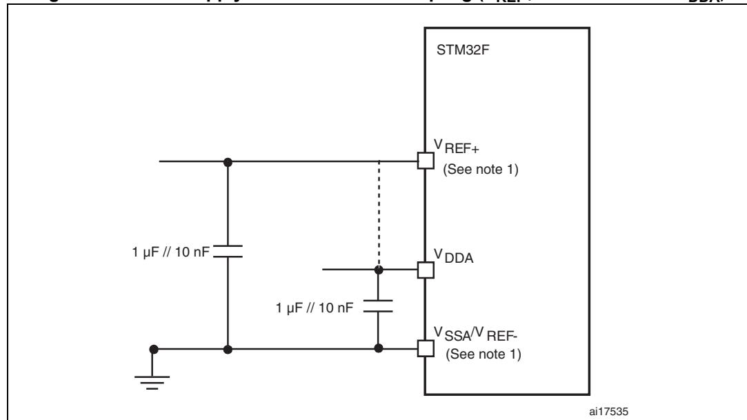
Figure 54. Power supply and reference decoupling ( V_{REF+} not connected to V_{DDA} )
