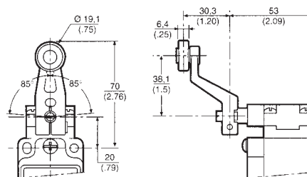
Offset Side Rotary Roller Lever A5A - Plastic Roller A5B - Metal Roller
