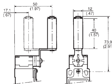
Side Rotary Conveyor Lever A9A Ceramic Roller
