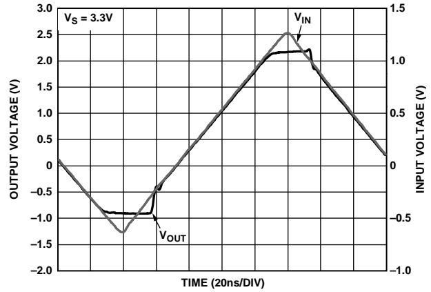
Figure 25. Output Overdrive Recovery
