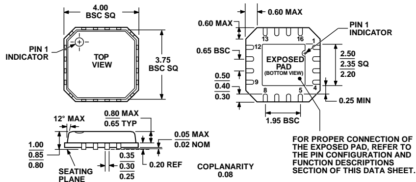
COMPLIANT TO JEDEC STANDARDS MO-220-VGGC Figure 49. 16-Lead Lead Frame Chip Scale Package [LFCSP_VQ] 4 mm x 4 mm Body, Very Thin Quad (CP-16-10) Dimensions shown in millimeters
