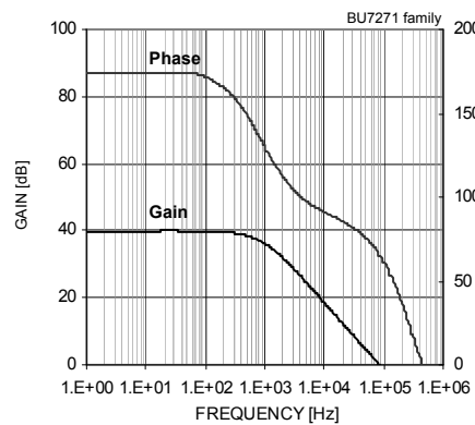
Fig. 46 Gain – Frequency
