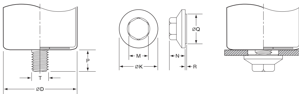
Type S: Stud Mounting Dimensions
