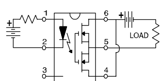
"C" Connection
