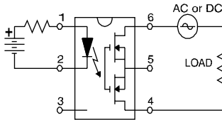
"A" Connection
