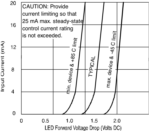
Figure 6. Input Characteristics (Current Controlled)
