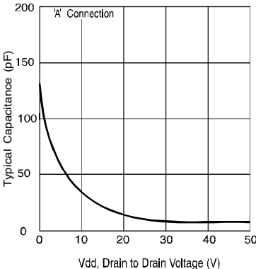
Figure 9. Typical Output Capacitance
