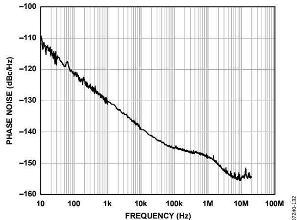
Figure 23. Additive (Residual) Phase Noise, CLK-to-CMOS @ 250 MHz, Divide-by-4
