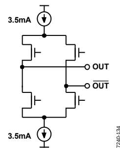
Figure 41. LVDS Output Simplified Equivalent Circuit with 3.5 mA Typical Current Source
