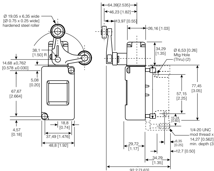
Figure 19. 206LS1 Dimensions
