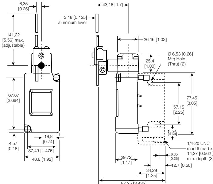
Figure 15. 202LS1 Dimensions
