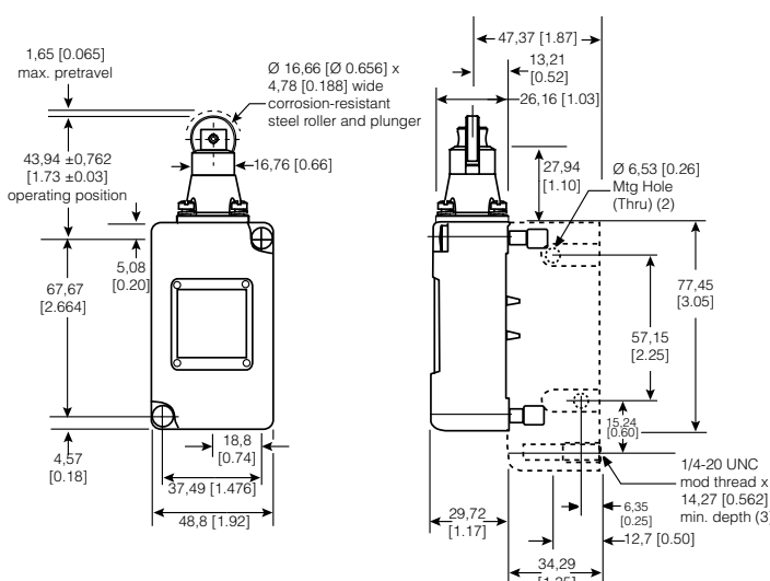
Figure 19. 206LS1 Dimensions
