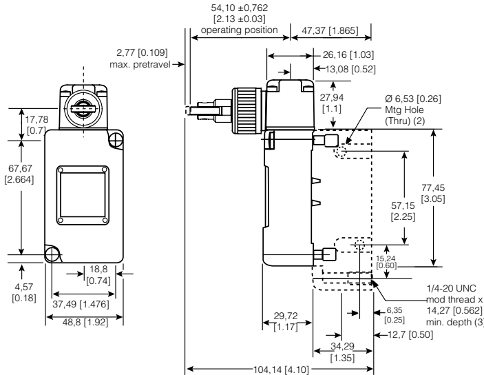
Figure 16. 203LS1 Dimensions
