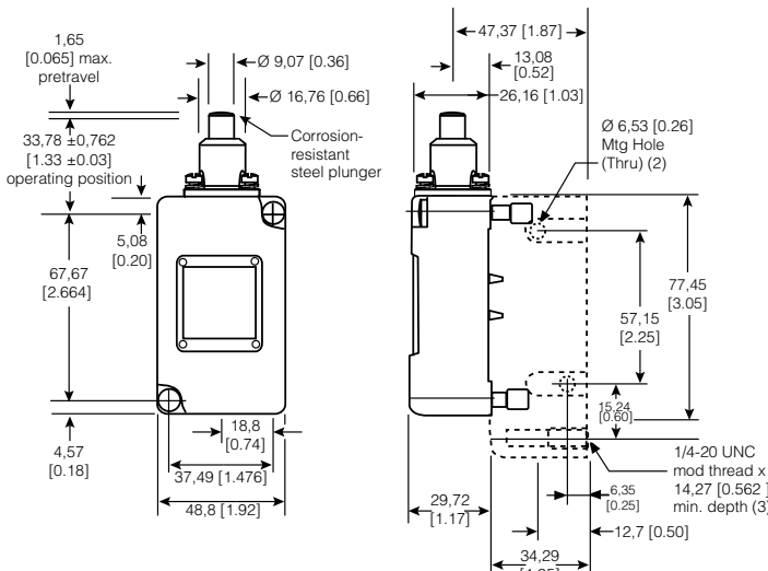
Figure 16. 203LS1 Dimensions
