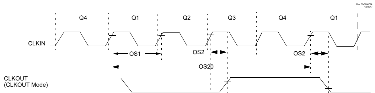
Figure 38-4. Clock Timing
