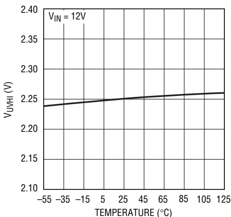
V_{UVHI} vs Temperature
