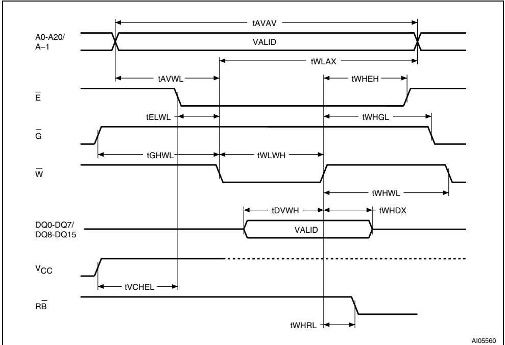
Figure 12. Write AC Waveforms, Write Enable Controlled
