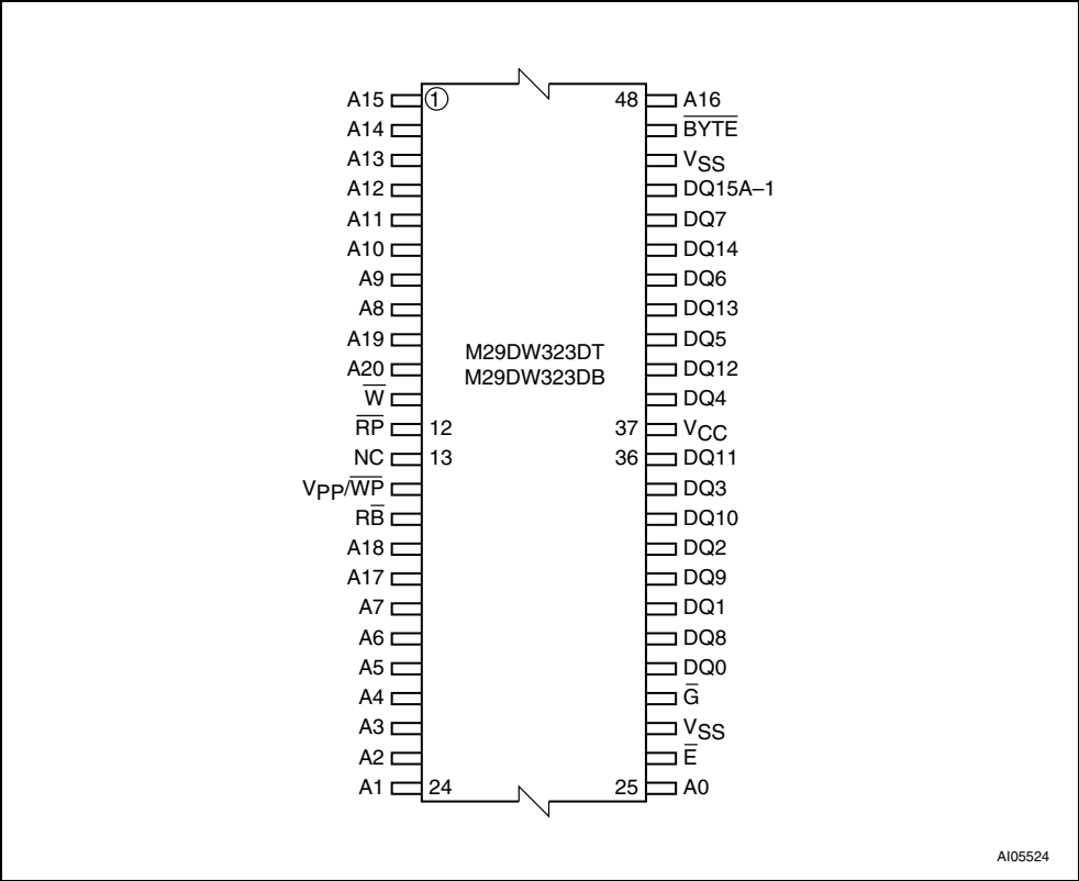
Figure 3. TSOP Connections
