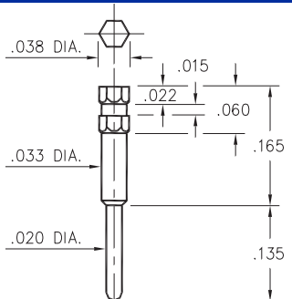
4366-0-00-XX-00-00-03-0 Hex press-fit in .034 plated thru hole
