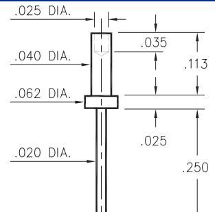
3147-3-00-XX-00-00-08-0 Swage mount in .043 hole. For .094 thick board.
