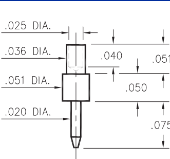
3135-1-00-XX-00-00-08-0 Swage mount in .040 hole. For .031 thick board.
