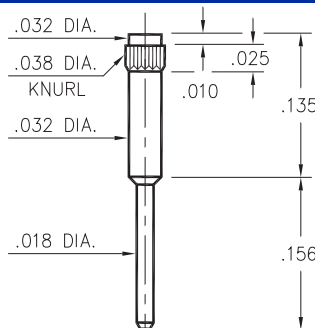
1267-0-00-XX-00-00-03-0 Press-fit in .035 mounting hole
