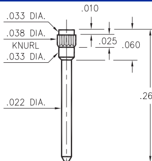
7827-0-00-XX-00-00-03-0 Press-fit in .035 mounting hole
