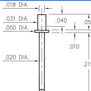
3129-1-00-XX-00-00-08-0 Swage mount in .035 hole. For .031 thick board.
