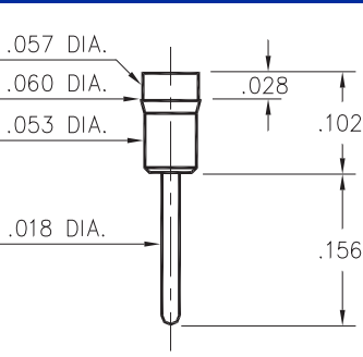
1130-0-00-XX-00-00-03-0 Press-fit in .057 mounting hole Pin material is Ph Br. 544 (B2)
