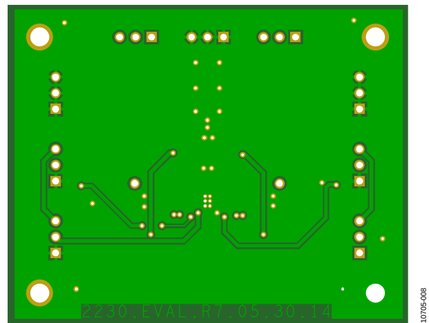
Figure 35. PCB Layout, Bottom
