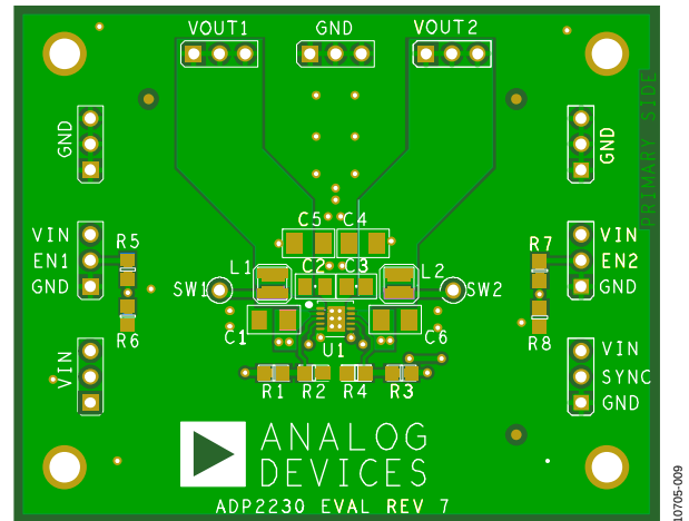
Figure 34. PCB Layout, Top
