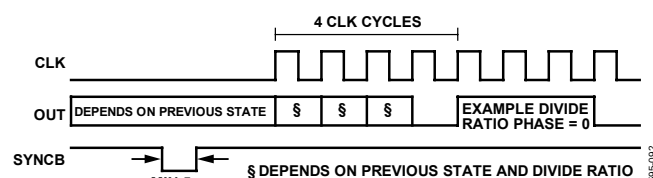
Figure 21. SYNCB Timing with No Clock Present
