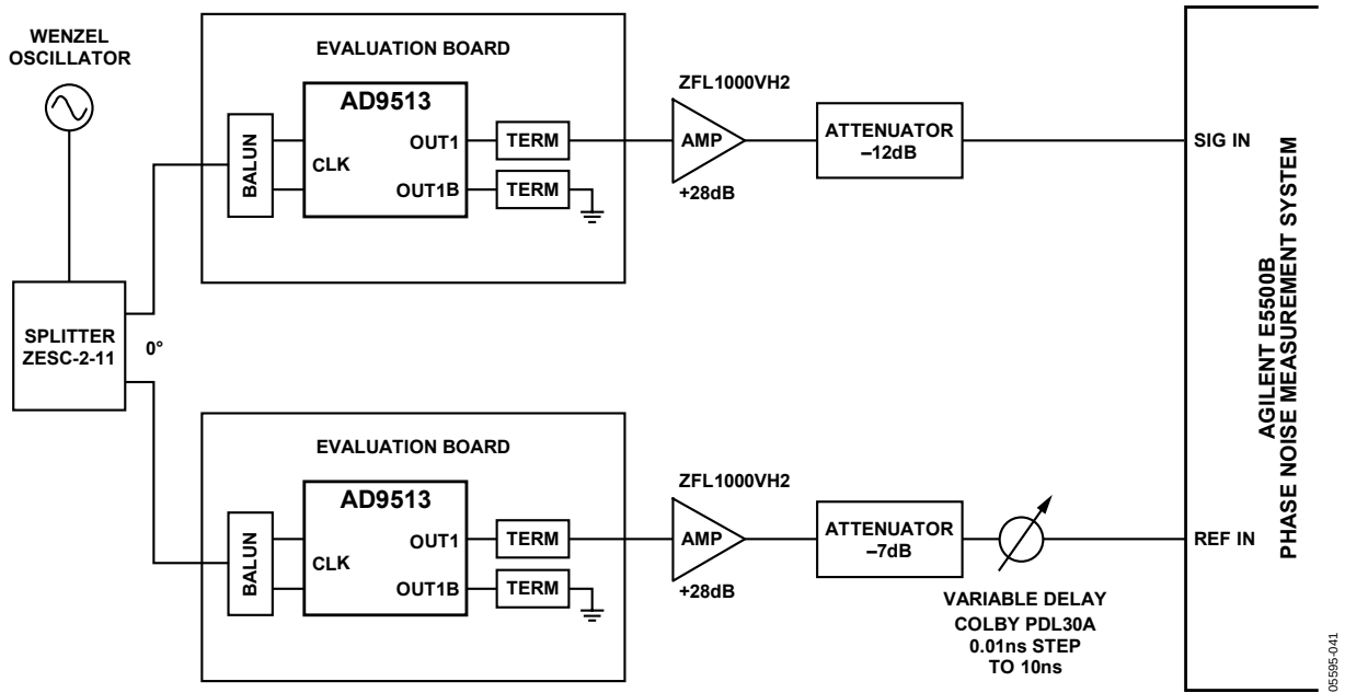
Figure 33. Additive Phase Noise Measurement Configuration
