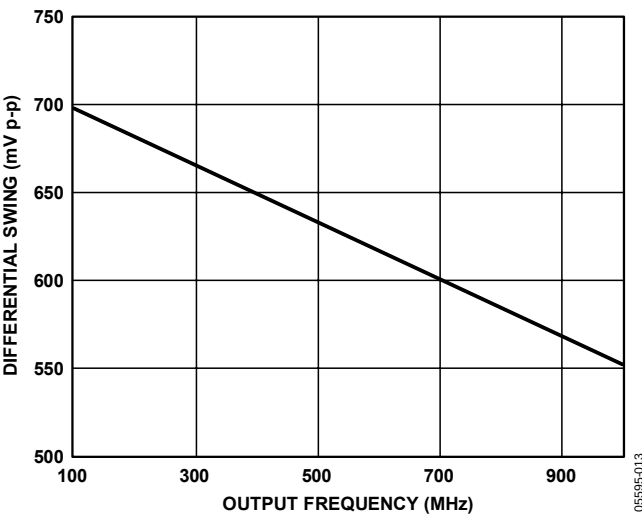
Figure 12. LVDS Differential Output Swing vs. Frequency
