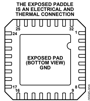
Figure 6. Exposed Paddle
