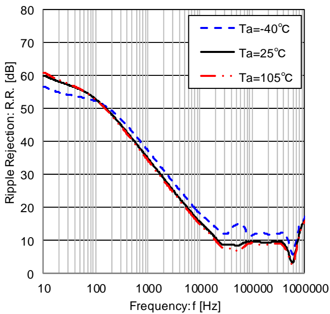
Figure 10. Ripple Rejection ( I_o=100\text{mA} )
