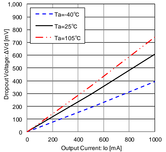
Figure 9. Dropout Voltage ( V_{cc}=4.75\text{V} ) ( I_o=0\text{mA} \rightarrow 1000\text{mA} )
